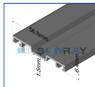
60 Gland Base
