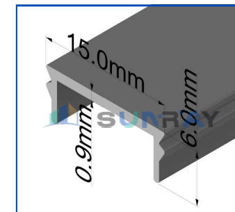
148 Universal Small Cover
