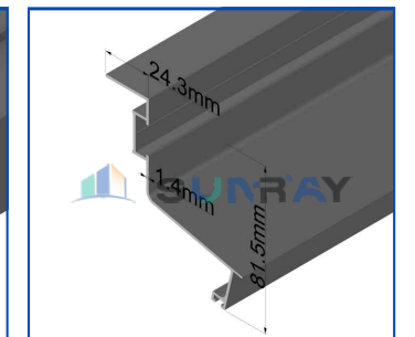
Soffit Stopper
