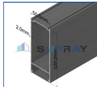
120-20 Main Beam
