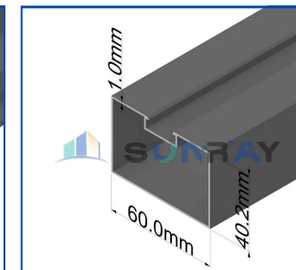
Waterproof Border
