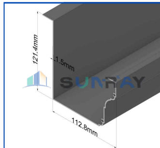
120 Sink
