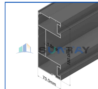
150 Decorative Beam
