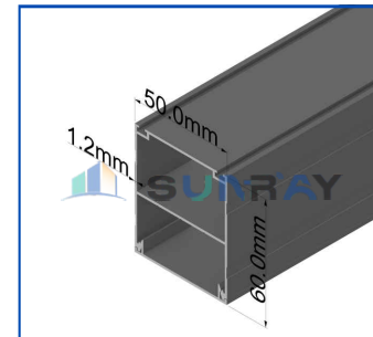
6050 Sub Girder
