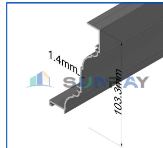
120 Sink Stacking Plate
