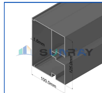
125 Decorative Beams
