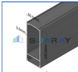
120-30 Main Beams
