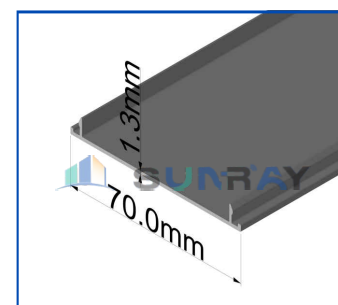
70 General Purpose Large Cover
