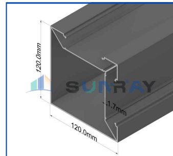
120 General Purpose Material - Column
